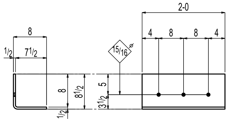
ONE BENT PLATE F-08.03M1
