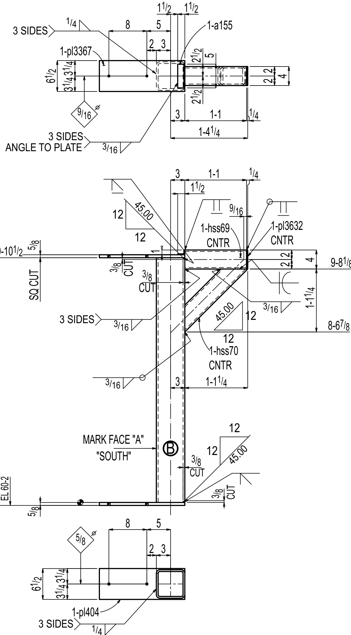
ONE COLUMN F-08.00C4
