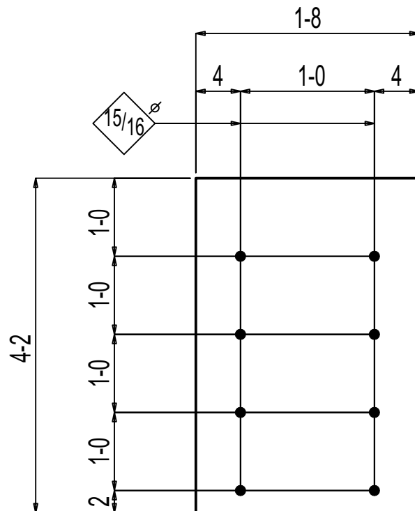
ONE EMBED PLATE F-08.03EP2
