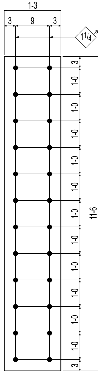
ONE EMBED PLATE F-08.03EP1
