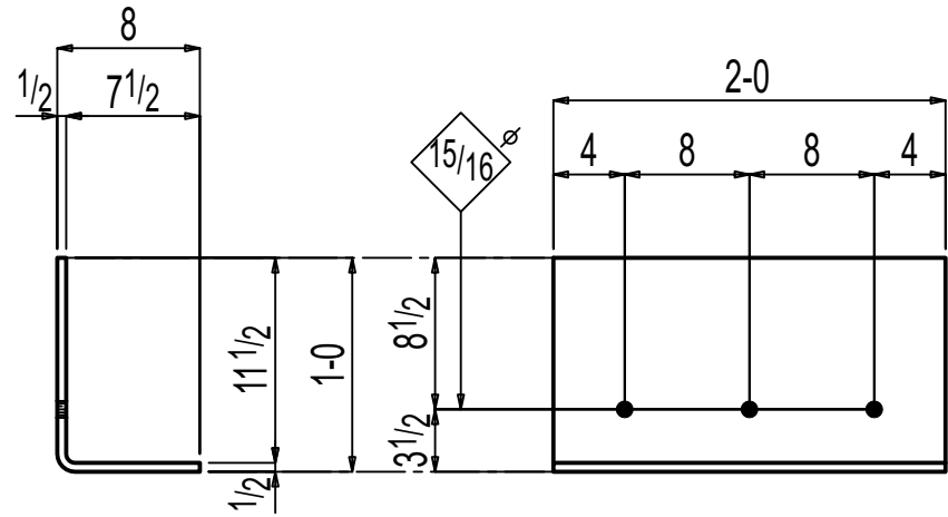
3 BENT PLATES F-08.03M2
