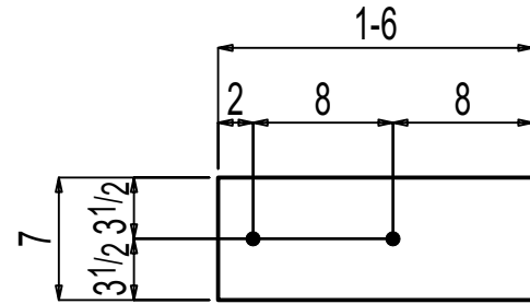
ONE LEVELING PLATE F-08.02LP1
